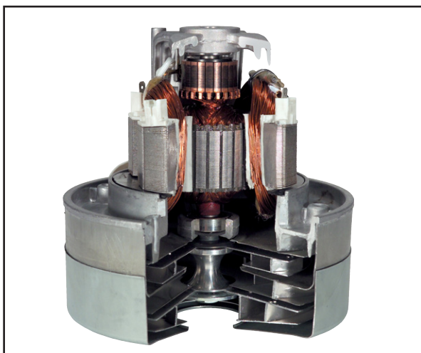
High Airflow Vacuum Motor
